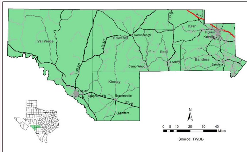
Figure 1-1. Location of the Plateau Region
