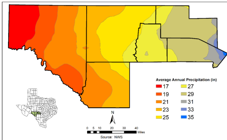
Figure 1-5. Variation of Precipitation
